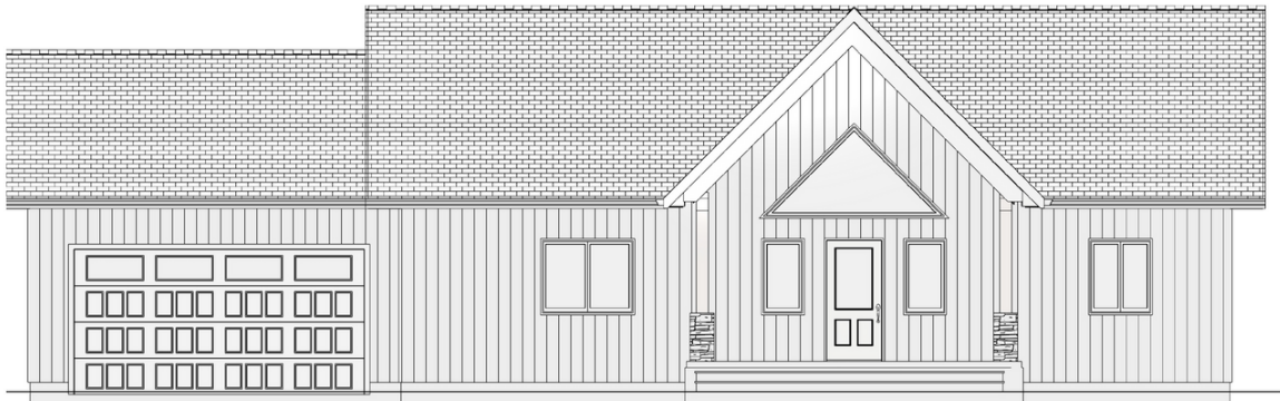
Front Elevation
